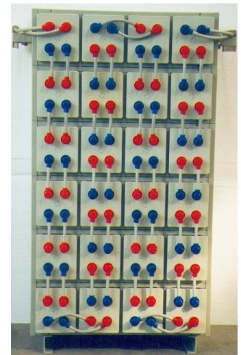
Six layer installation of GTS-600E cells for 48V system
